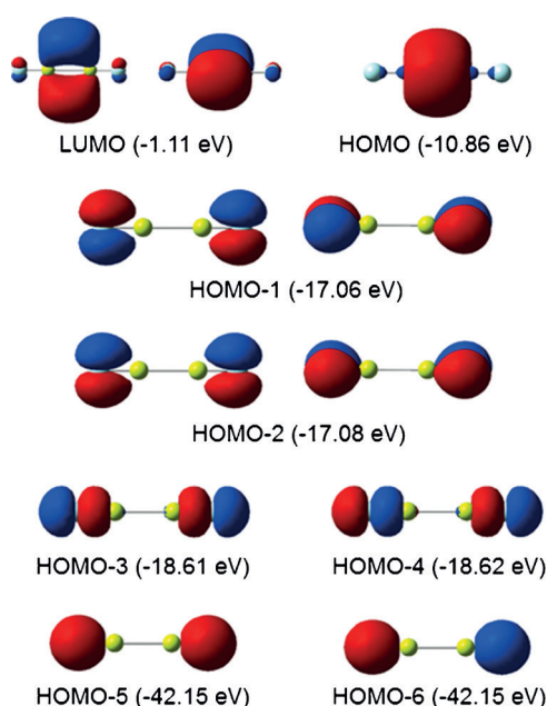
Figure 3. Shapes and eigenvalues of the lowest unoccupied MO (LUMO) and the relevant occupied valence orbitals of Be 2 F 2 .
