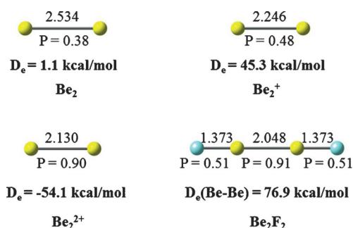
Figure 2. Bond lengths [Å] of Be 2 , Be 2 + , Be 2 2+ , and Be 2 F 2 calculated at the CCSD(T)/cc-pVTZ level of theory. Wiberg bond order P determined using the CCSD/cc-pVTZ densities at the above geometries. Bond dissociation energies D e of the Be–Be bonds at the CCSD(T)/cc-pVTZ level of theory.
