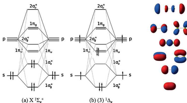
Figure 1. Orbital correlation diagrams for a) the X 1 Σ g + ground state and b) the (3) 1 Δ g excited state of Be 2 and shape of the MOs.
